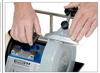
Fig. 3.2: long Knife Jig SVM-140
