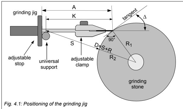
Fig. 4.1: Positioning of the grinding jig
